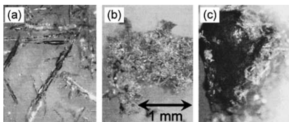
Figure 3. The photomicrographs of the silver dendrite. (a) the outside of the bore tube (control), (b) the bottom position (9.3 T, 980 T 2 /m), (c) the top position (5.6 T, -940 T 2 /m).
