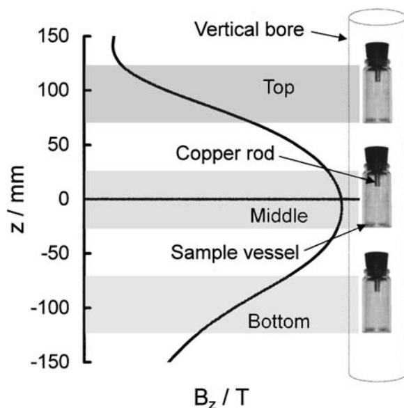
Figure 1. The distribution of the vertical magnetic field B(z) . z is the distance from the center of the magnetic field (15 T) along the magnetic axis. The gray parts show the area of the magnetic fields where the sample vessels were placed. These positions shall be called top, middle, and bottom from the top. The right-hand vertical bore's picture corresponds to the plot of distribution of the magnetic field.
