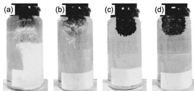
Figure 2. The photographs of silver dendrites after 2 h reaction. (a) the outside of the bore tube (control, <0.0005 T), (b) the bottom position (9.3 T, 980 T 2 /m), (c) the middle position (15 T, -160 T 2 /m), (d) the top position (5.6 T, -940 T 2 /m).
